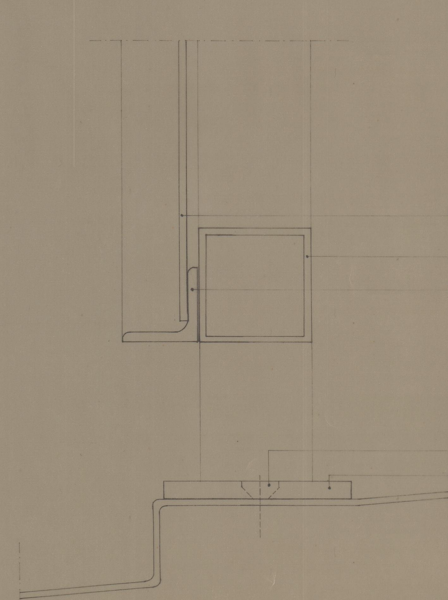
CORTE VERTICAL
