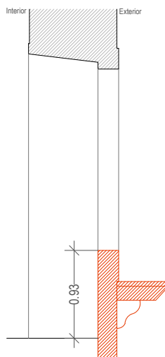
Corte Vertical
