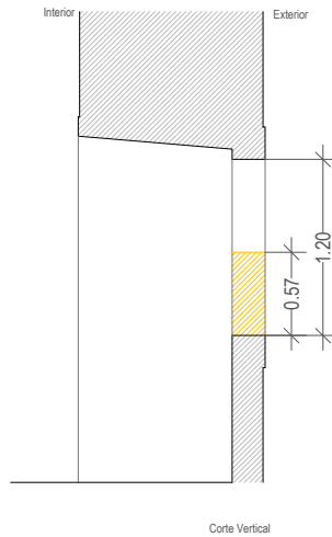
Corte Vertical
