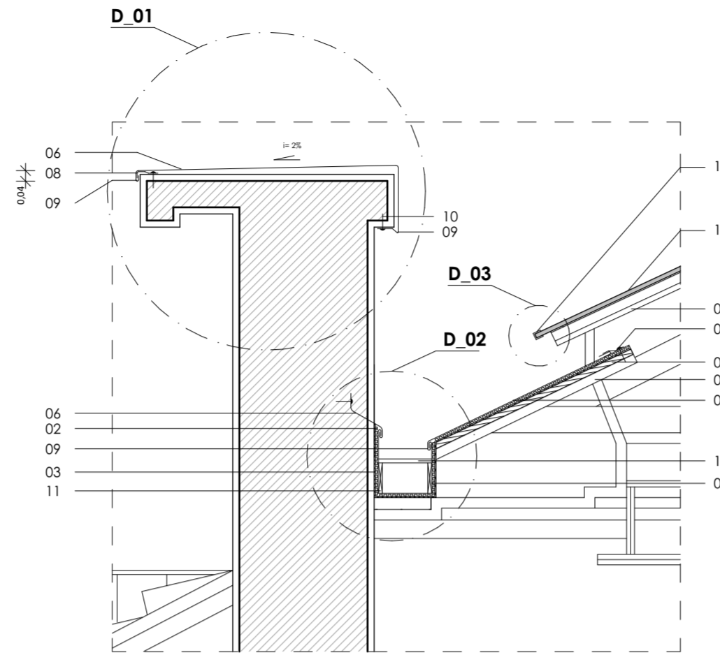
P_02 esc: 1/20
